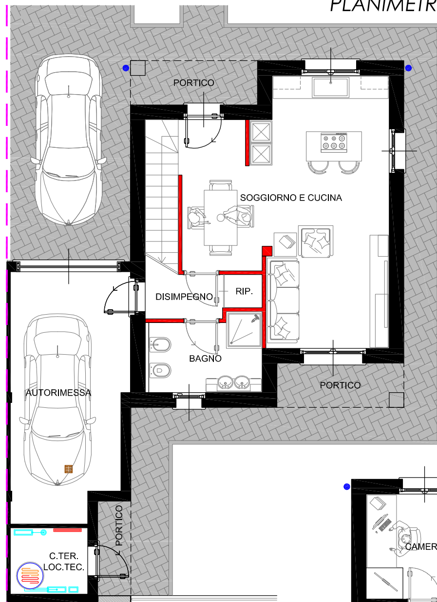
PLANIMETRIA PIANO TERRA
