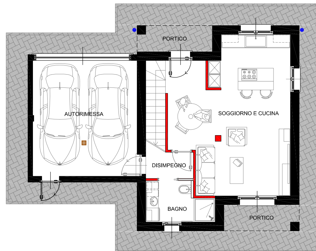
PLANIMETRIA PIANO TERRA
